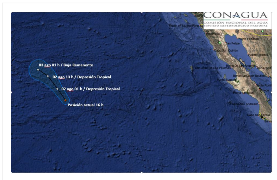
Trajectory forecast of the Tropical Depression "Irwin"
